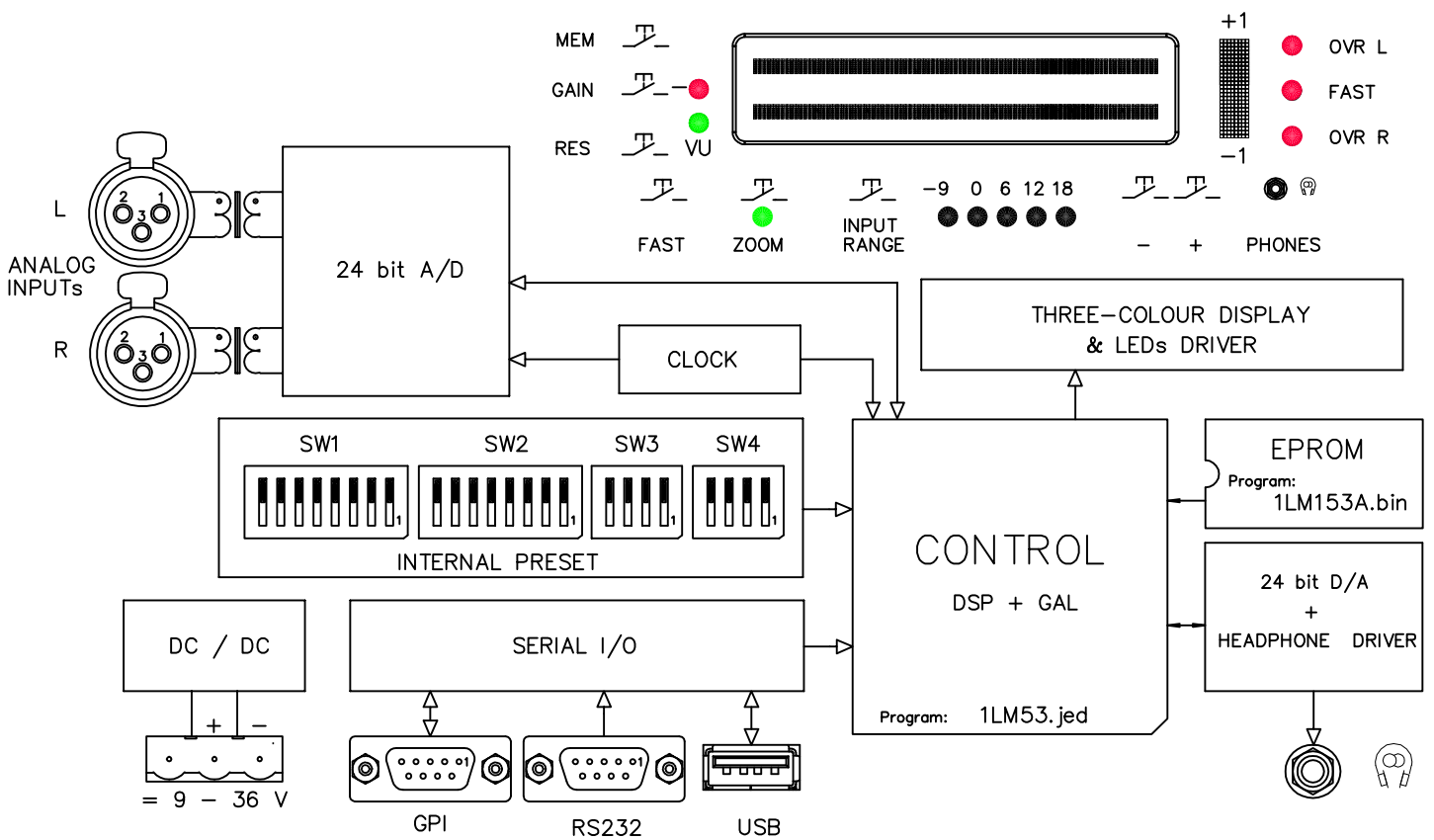
BLOCK DIAGRAM 1LM153A
